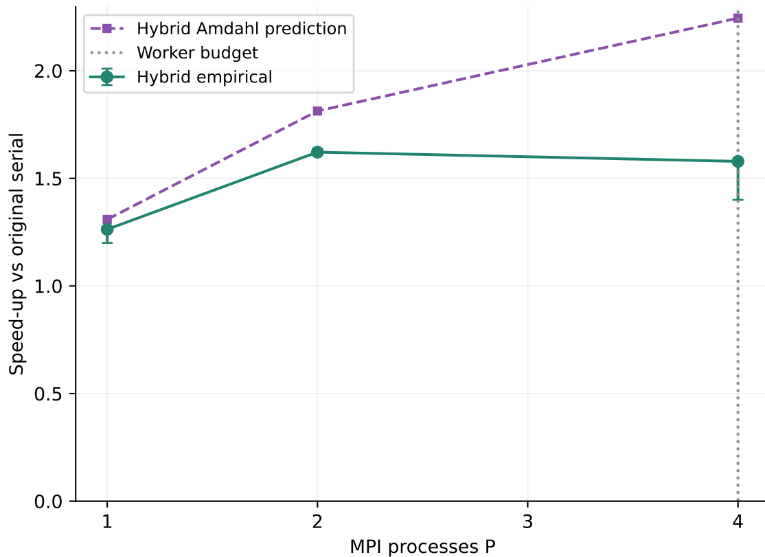
Fixed H=2
