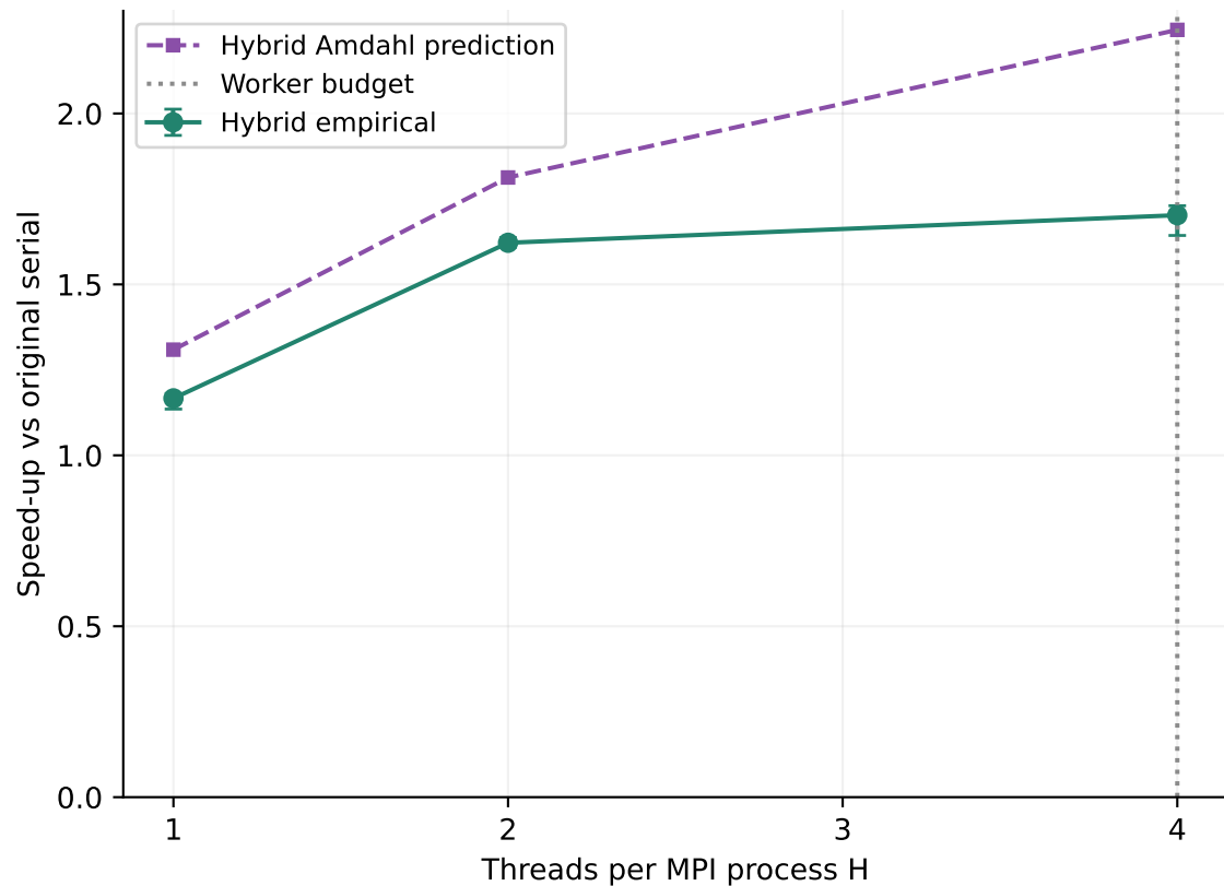
Fixed P=2
